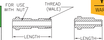
Fig 1 THREADED
