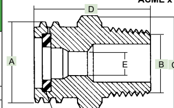
Gasket (Furnished with adapter)
