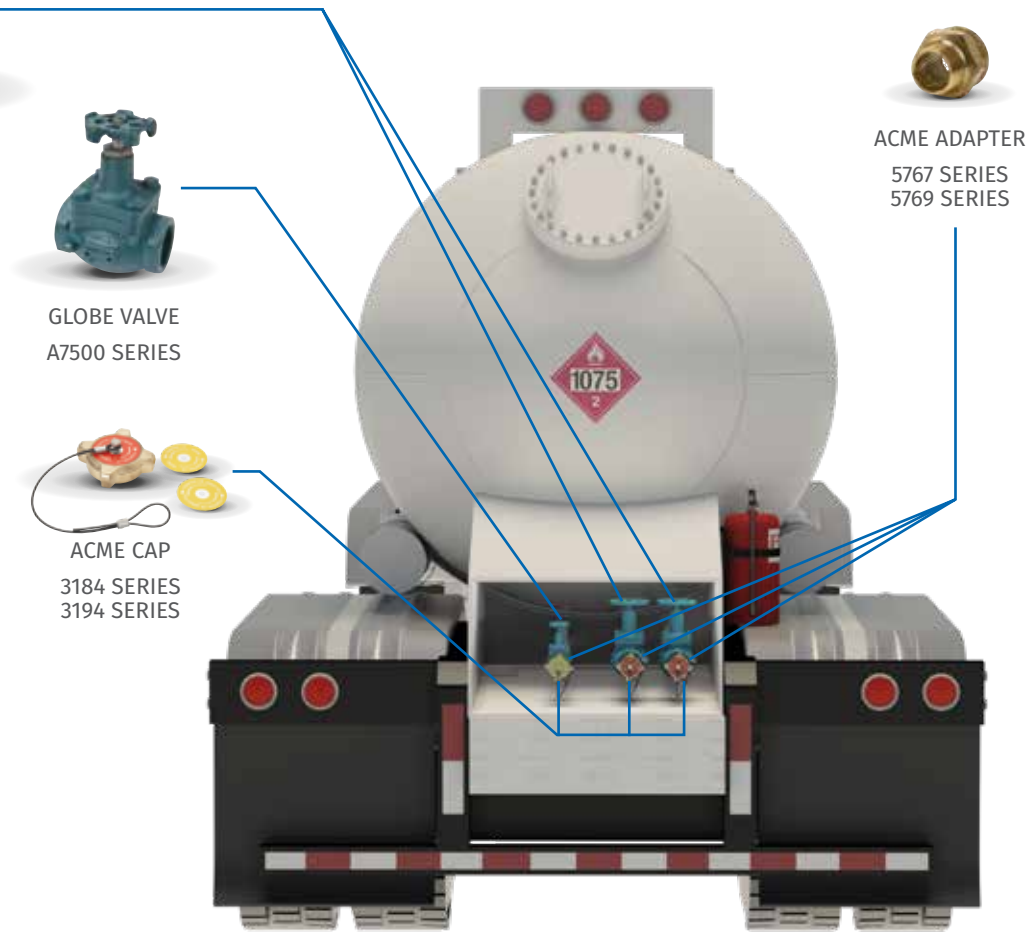
GLOBE VALVE A7500 SERIES
