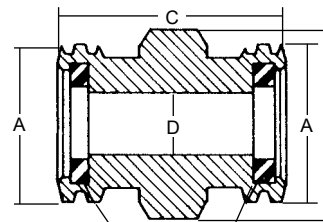
Gasket (Furnished with adapter)
